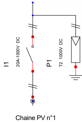
FRONIUS 3.6 - PV
