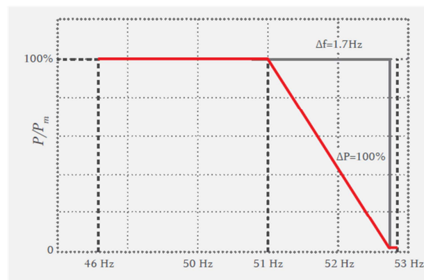
Figure 3: Schematic depicting GFdPR strategy to ensure secure energy supply
