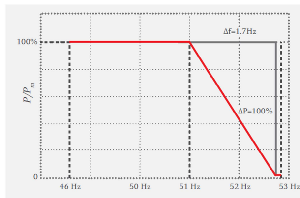
/ Frequency droop function of Fronius inverters with MicroGrid setup. Fully adjustable to harmonise perfectly with the Inverter-Charger.
