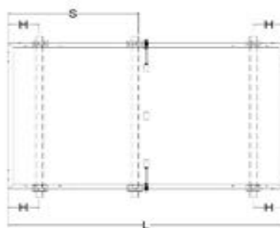
Figure 26 Bride-C
