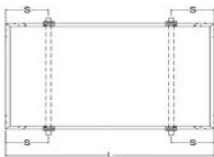
Figure 25 Bride-A
