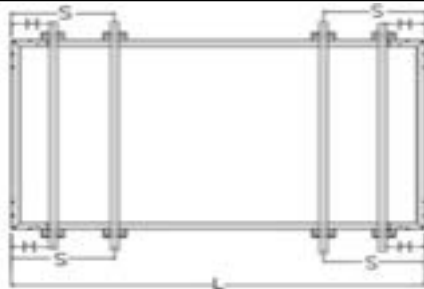
Figure 14 Bride-I
