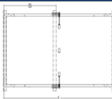
Figure 28 Bride-G
