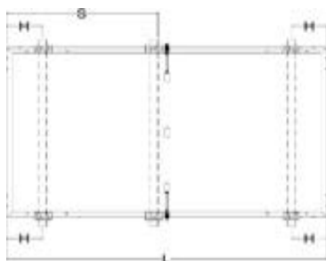
Figure 8 Bride-C
